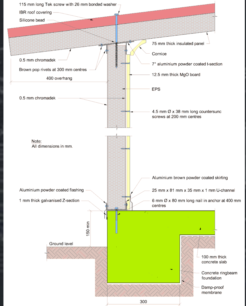
Figure 1: Vertical section through external wall with foundation detail
