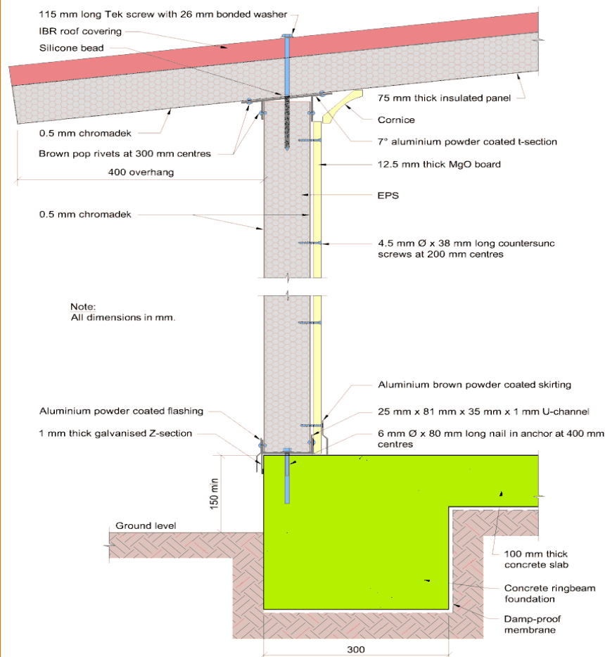
Figure 1: Vertical section through external wall with foundation detail
